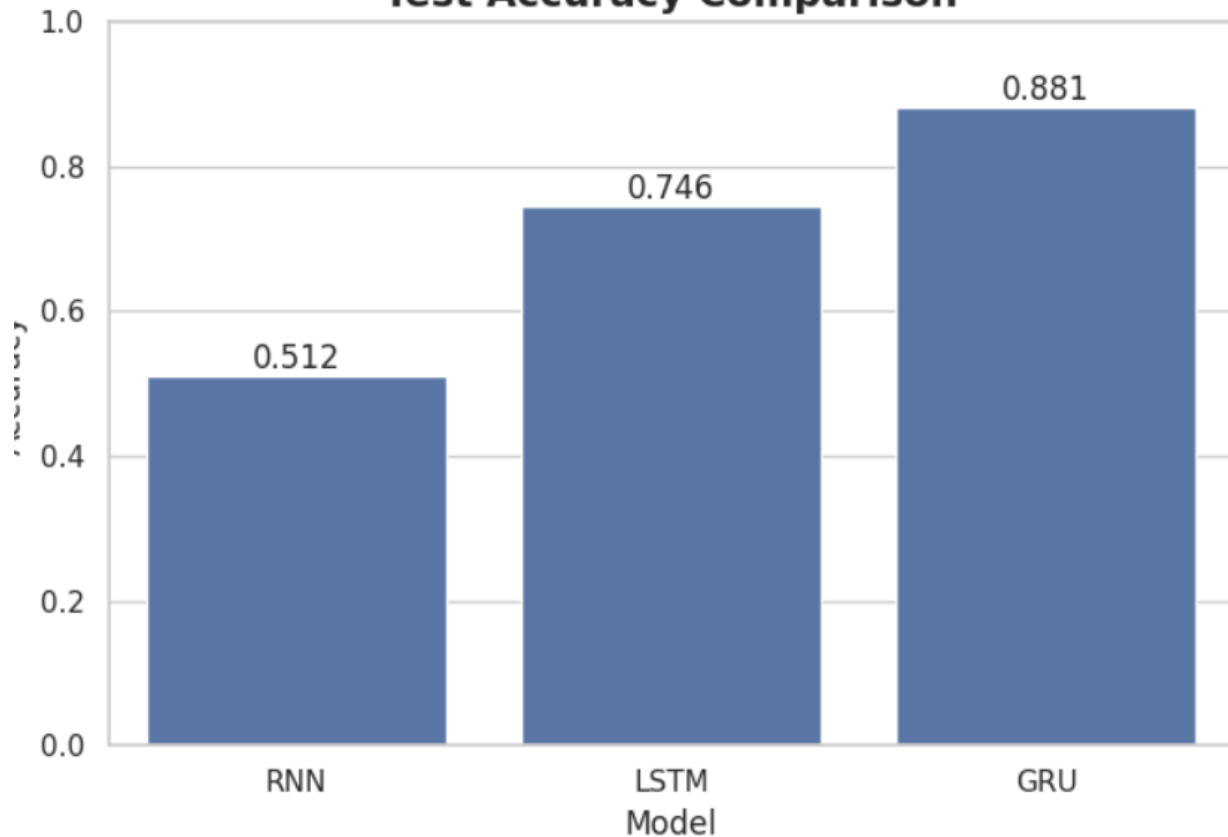
Test Accuracy Comparison
