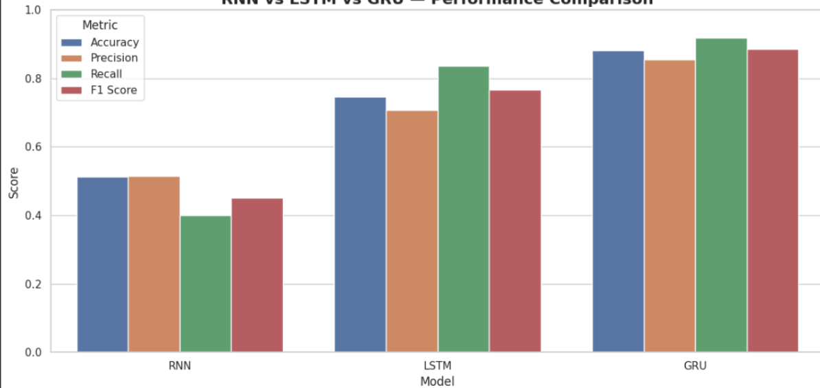
Test Accuracy Comparison
