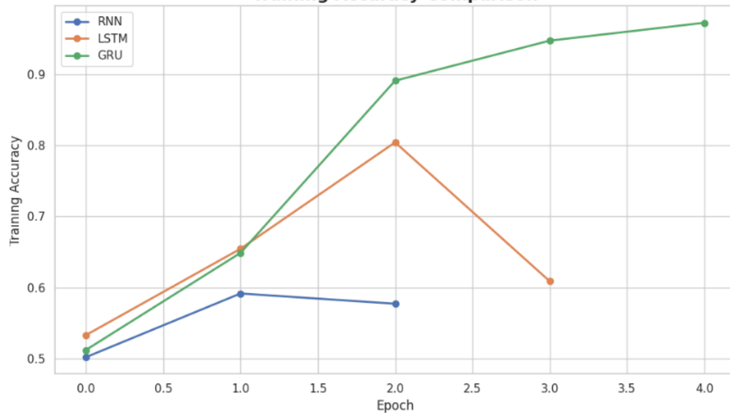
Training Accuracy Comparison
